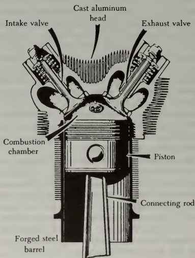
FIGURE 1-14. Cutaway view of the cylinder assembly.
